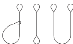
Choker Vertical Basket
